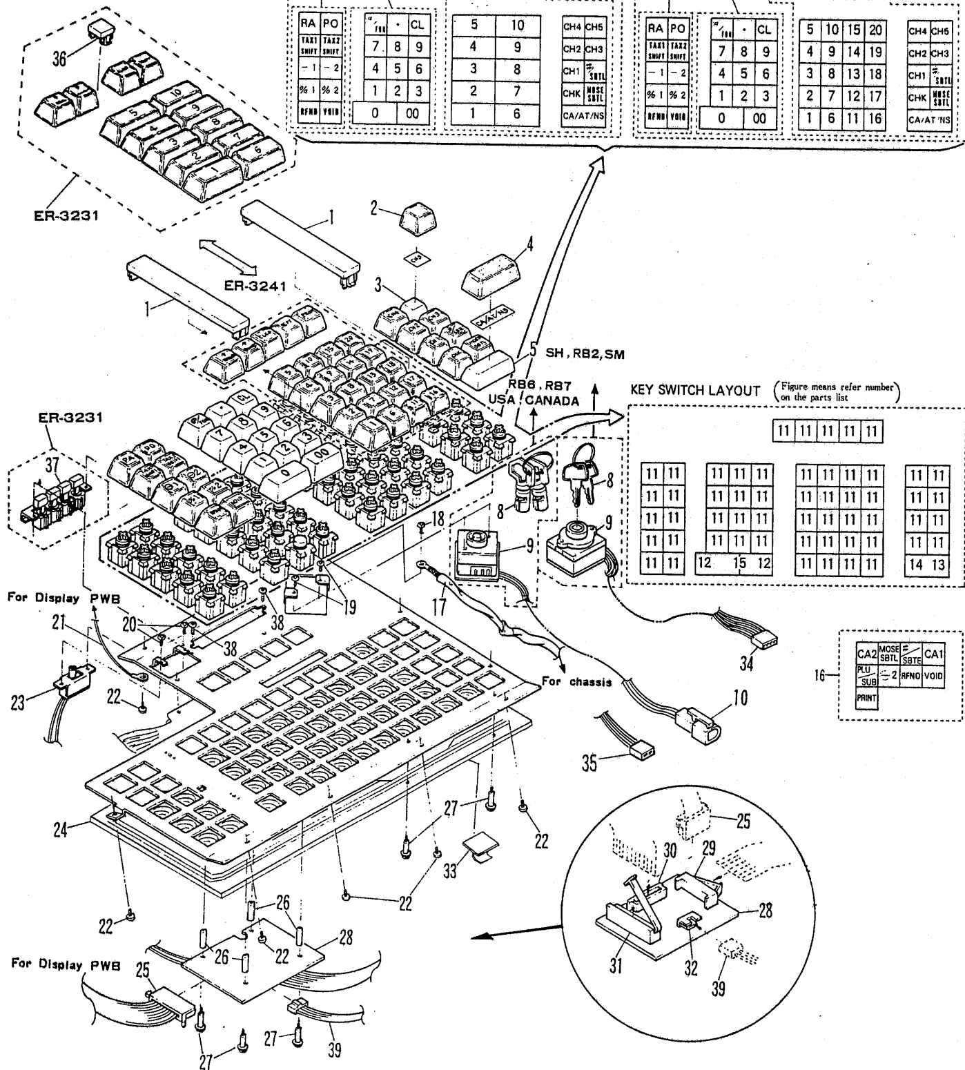
ER-3241 KEY TOP & KEYPAD LAYOUT
