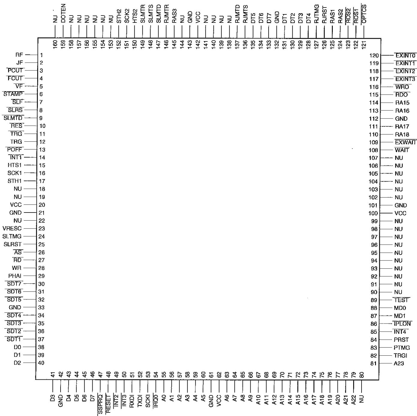
GATE ARRAY (F258016PC) MPCA5
